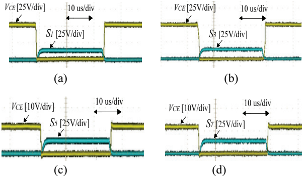
Fig. 11. Operating waveforms of driving signals and switching terminal voltages when U_2 = 12\text{V} and P = 10\text{ W} : (a) S_1 ; (b) S_3 ; (c) S_5 ; (d) S_7 .
