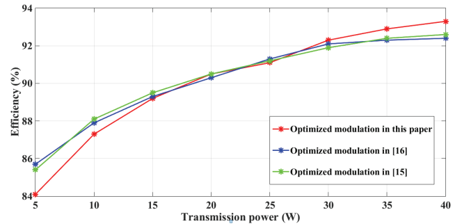
Fig. 14. Efficiency curves varied with the transmission power in different optimized modulation with U_2 = 12\text{ V} .
