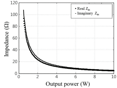
Fig. 5. Correlation between impedance and output power.
