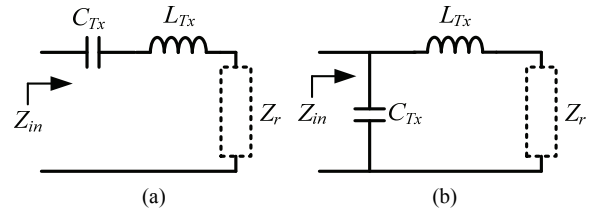
Fig. 4. Loaded equivalent circuit according to the Tx resonator type. (a) Series type of Tx. (b) Parallel type of Tx.
