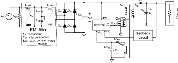
Fig. 9. Structure of a conventional AC/DC travel adapter [28].
