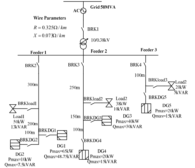
Fig. 9. Topology of a microgrid.
