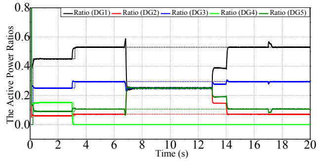
Fig. 14. Active power ratios of DGs.
