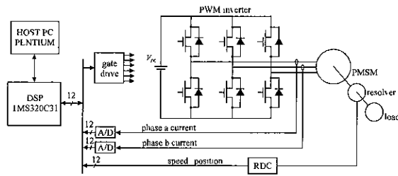
Fig 4 Configuration of experimental system
