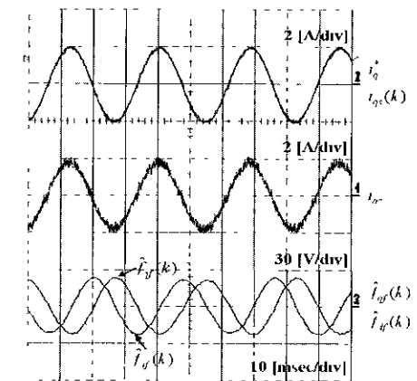
(d) Proposed control under \Delta\lambda_m = -0.5\lambda_{m0}
