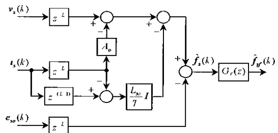
Fig 1 Disturbance estimation using time delay control approach
