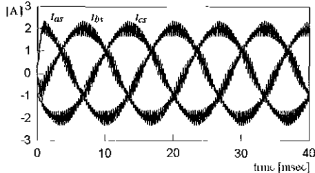
(b) PI decoupling control for the nominal parameters
