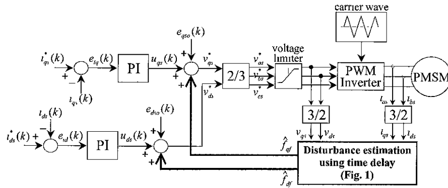
Fig 3 Overall block diagram for the proposed current control scheme
