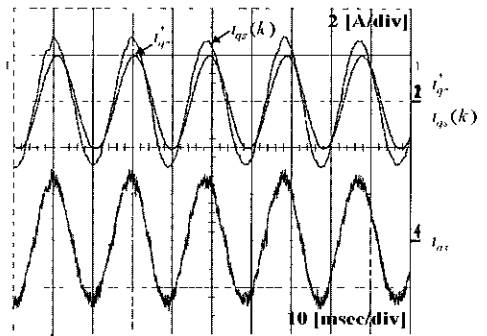
(c) PI decoupling control under \Delta\lambda_m = -0.5\lambda_{m0}
