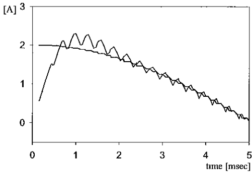
(b) Predictive plus time delay estimator in synchronous frame [Ref 13]
