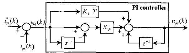
Fig 2 Digital implementation for the q -axis PI controller using the backward difference method
