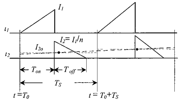
(b) Current waveforms at the primary and the secondary side of the flyback transformer
