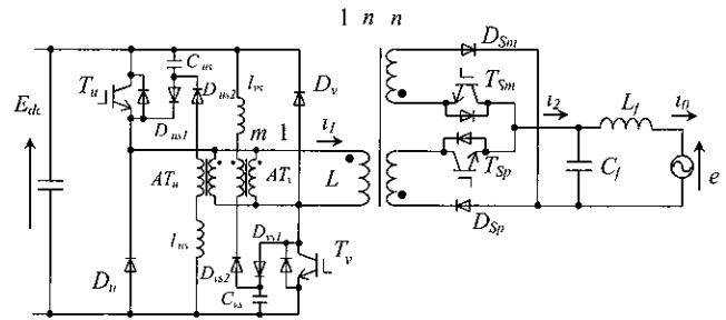
Fig 5 Flyback transformer linked high-frequency soft-switching sinewave inverter using energy regenerating snubber circuit
