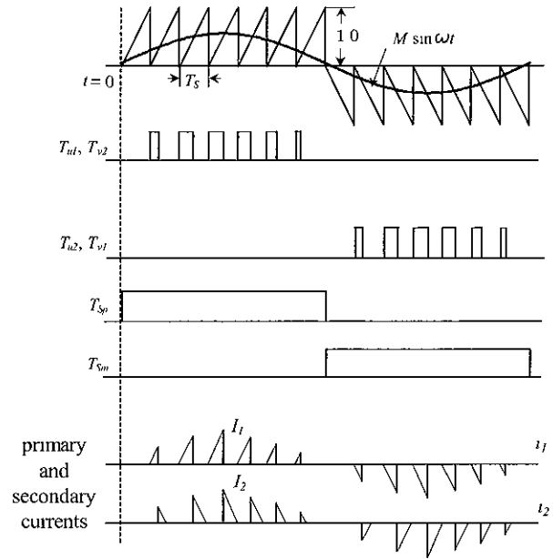
(a) Gate control pulse signals
