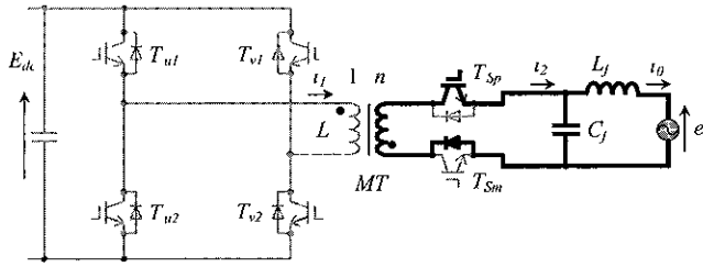
(b) Turn-off mode of DC side active power switches T_{u1} and T_{v2}
