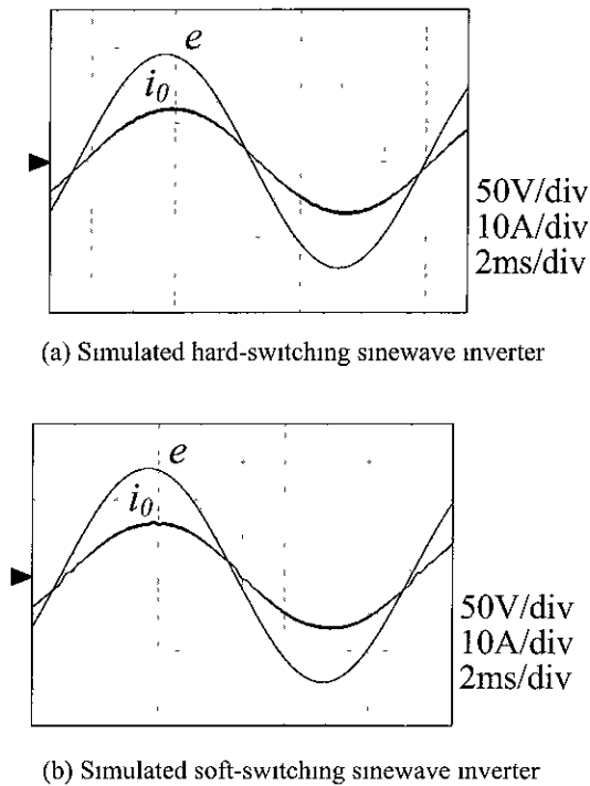
Fig 10 The computer simulated voltage and current waveforms of the sinewave inverter
