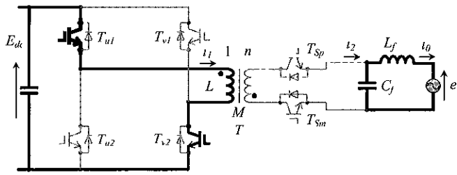
(a) Turn-on mode of DC side active power switches T_{u1} and T_{v2}
