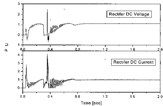
(c) Rectifier's voltage and current at three phases fault
