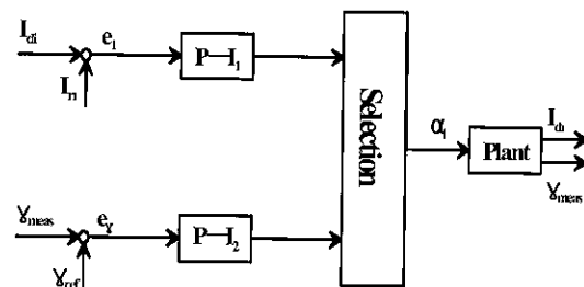
(a) Original Inverter control
