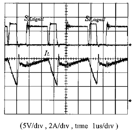
Fig 17 The experimental result by the condition of the Eq (2)
