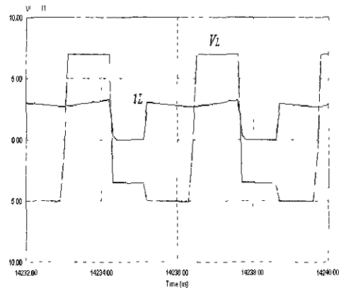
(a) Voltage and current of the primary side of the transformer
