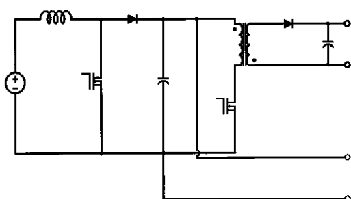
(b) Boost and Flyback converter
