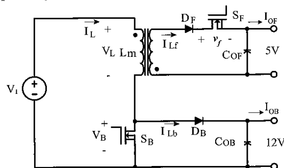
Fig 2 The proposed PWM DC/DC converter circuit
