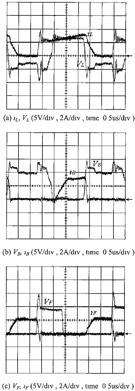
Fig 15 The key voltage and current waveforms of the proposed converter
