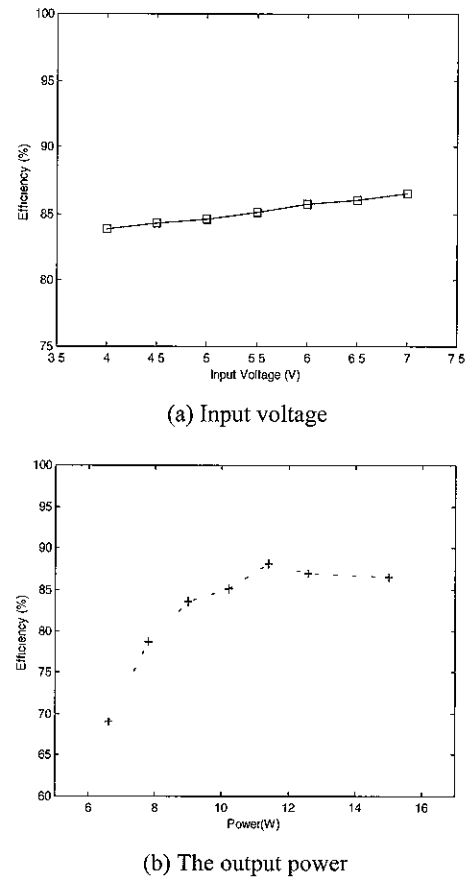
Fig 16 Experimentally measured efficiency
