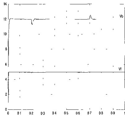
(a) At the variation of the input voltage
