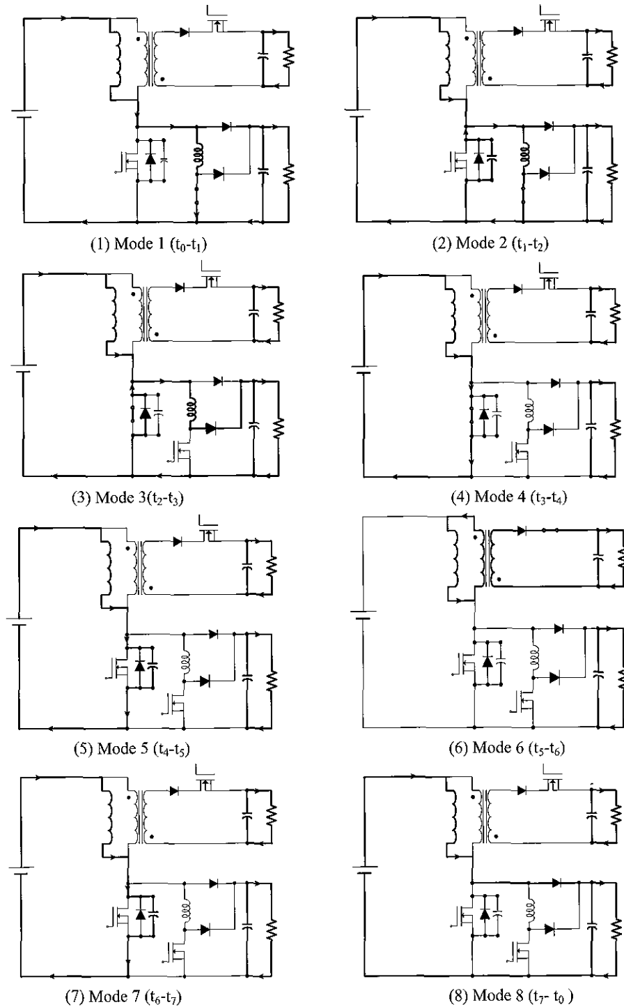
Fig 6 Eight topological operation stages of the proposed converter
