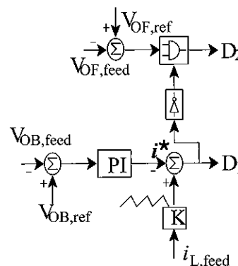
Fig 7 The overall system block diagram
