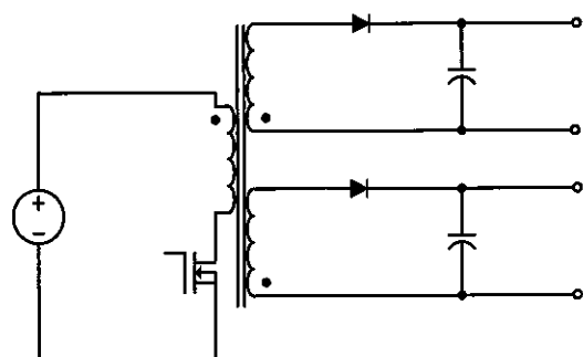
(a) Flyback converter with multi-winding
