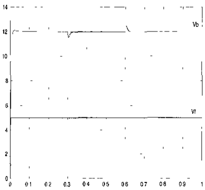
(c) In case of the load change of the lower converter
