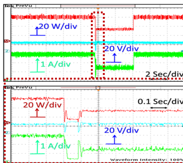
Fig. 13. Incremental Conductance result with reduction in Radiation G from 1000 to 900 to 1000 W/m 2 .
