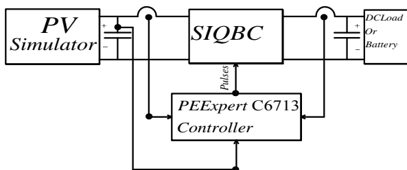
Fig. 10. Schematic of the Experimental Setup.
