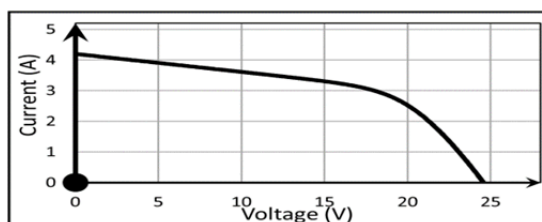
Fig. 12. Programmed PV specifications.
