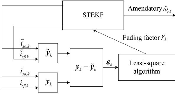
Fig. 2. Speed estimation structure based on LS-STEKF.
