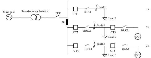
Fig.1. A typical Microgrid system.
