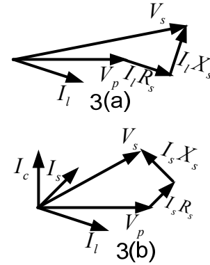
Fig. 3. Phasor diagram (a) without D-STATCOM (b) with D-STATCOM.
