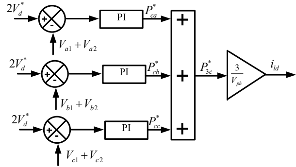
Fig. 4. Calculation of compensator powers.
