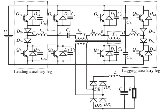
Fig. 4. Topology of the dual-active soft-switching converter.
