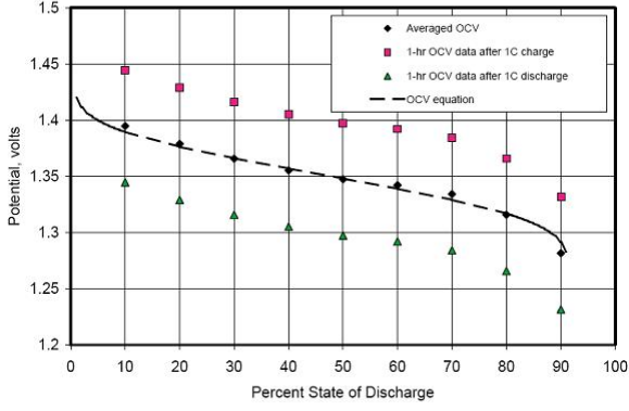
Fig. 6. Average OCV for charge and discharge [9].
