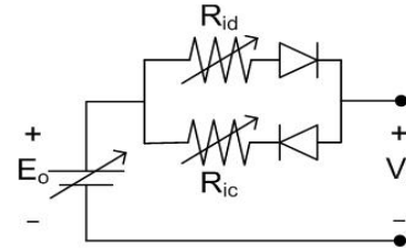
Fig. 5. Modified battery model.
