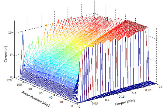
(b) Look-up table of the current reference.
