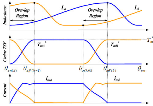
(a) Torque sharing function and current waveform.
