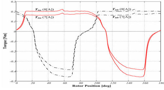
(a) Torque profile of the proposed motor.
