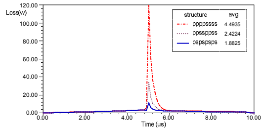
Fig. 14. Simulated winding loss with different structures in time domain with current excitation given in Table I.
