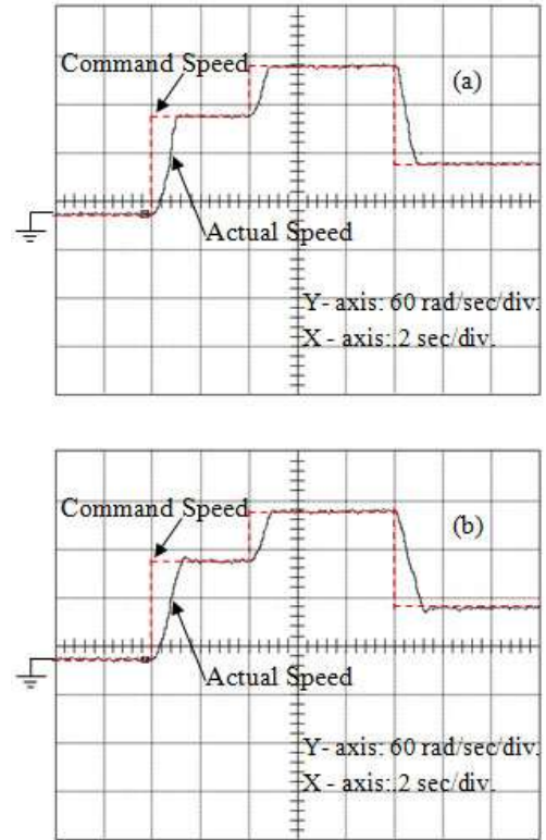
Fig. 16. Experimental speed response step change in command speed (120 rad/ sec to 180 rad/sec and again to 60 rad/sec) for (a) wavelet fuzzy based controller and (b) PI controller.
