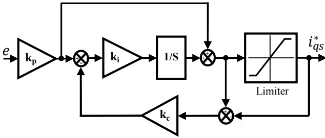
Fig. 3. Structure of PI Controller with Anti-windup.
