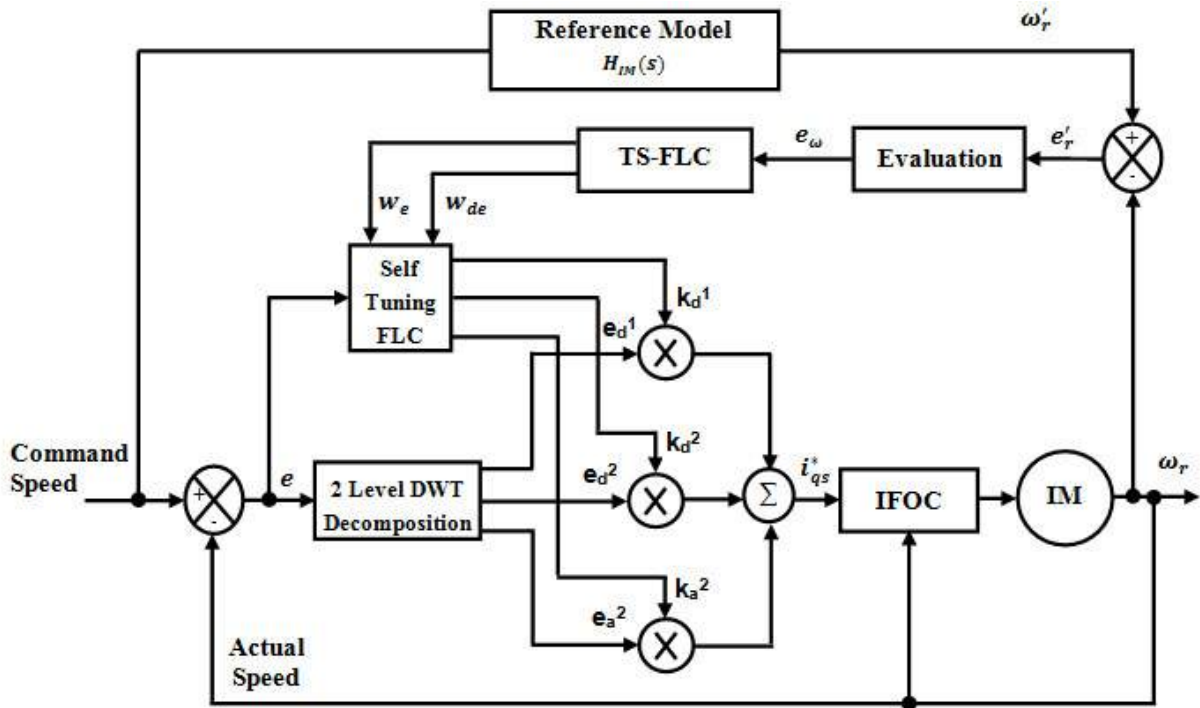
Fig. 5. Schematic of the wavelet-fuzzy based self tuning controller for IFOC of Induction motor drive.
