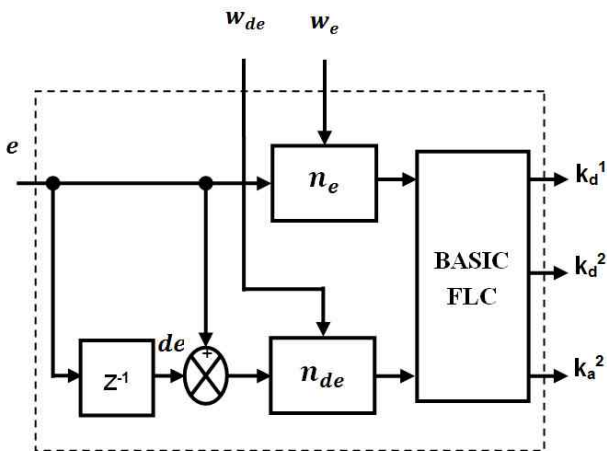
Fig. 6. Structure of Self-Tuning FLC Block.
